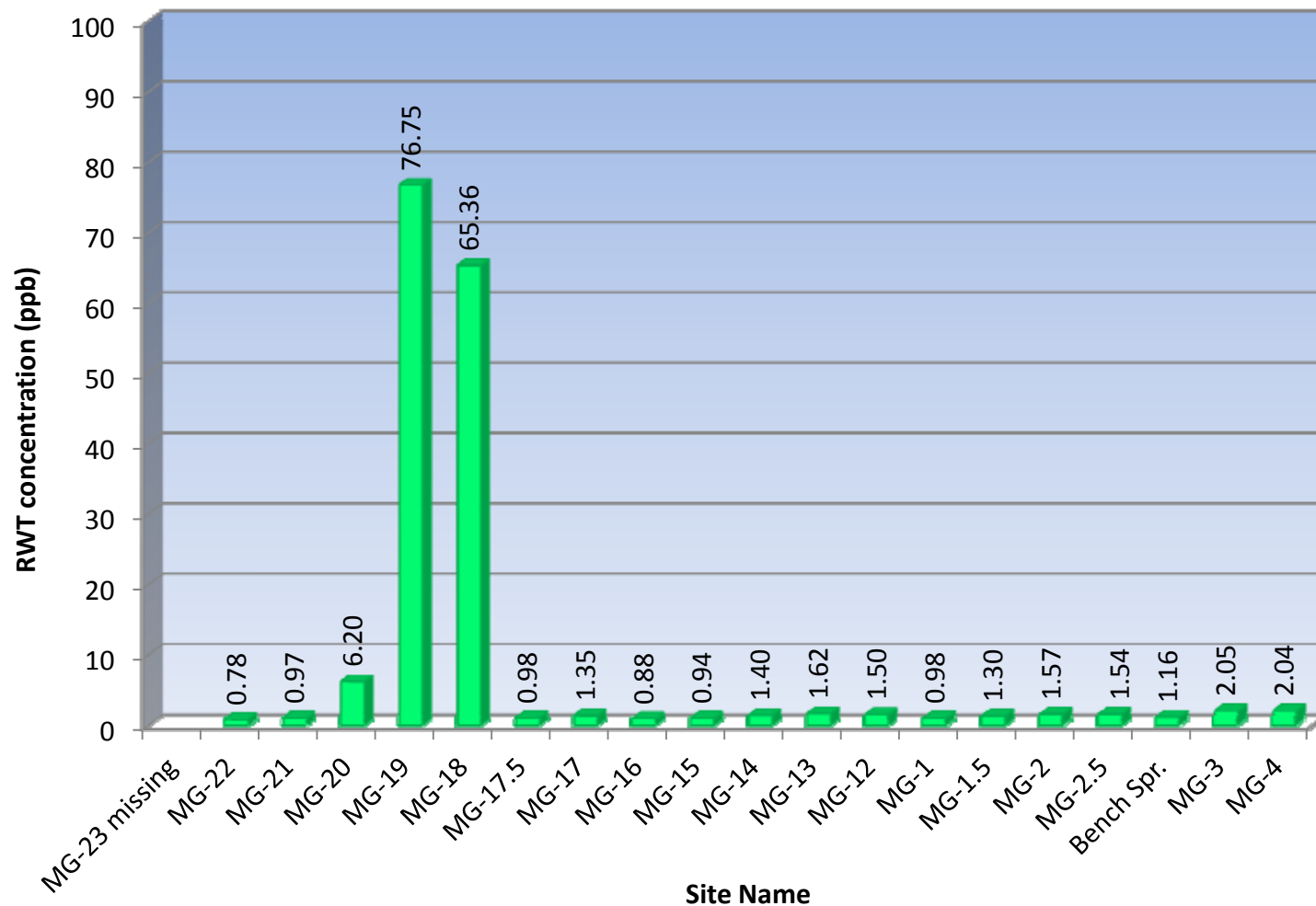
Figure 23. Graph of results from charcoal packets for N. Riddle well #25 Rhodamine WT trace. Dye was detected with positive results at sites MG-18, 19 and 20 at about 50 to 70 times above the ambient background fluorescence with the remaining sites negative. MG-23 was missing.
