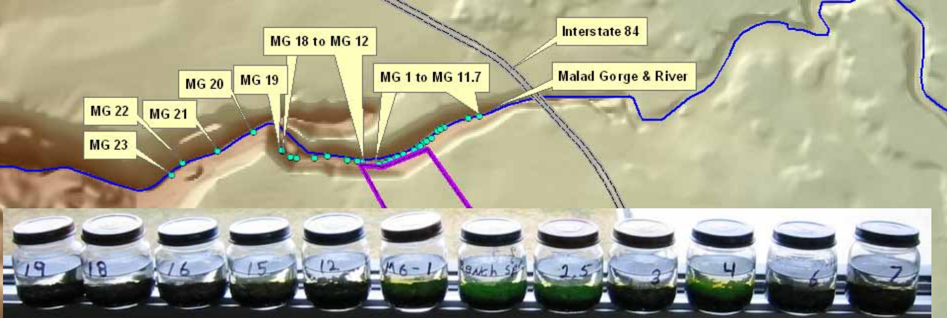
Figure 16. Visual results of charcoal packet analysis from Trace #1 showing Fluorescein dye in MG-1, 2.5, 4 and the Bench Spring. The packet at MG-3 had shifted out of the water. Trace #1 was started during winter conditions in the Gorge.
