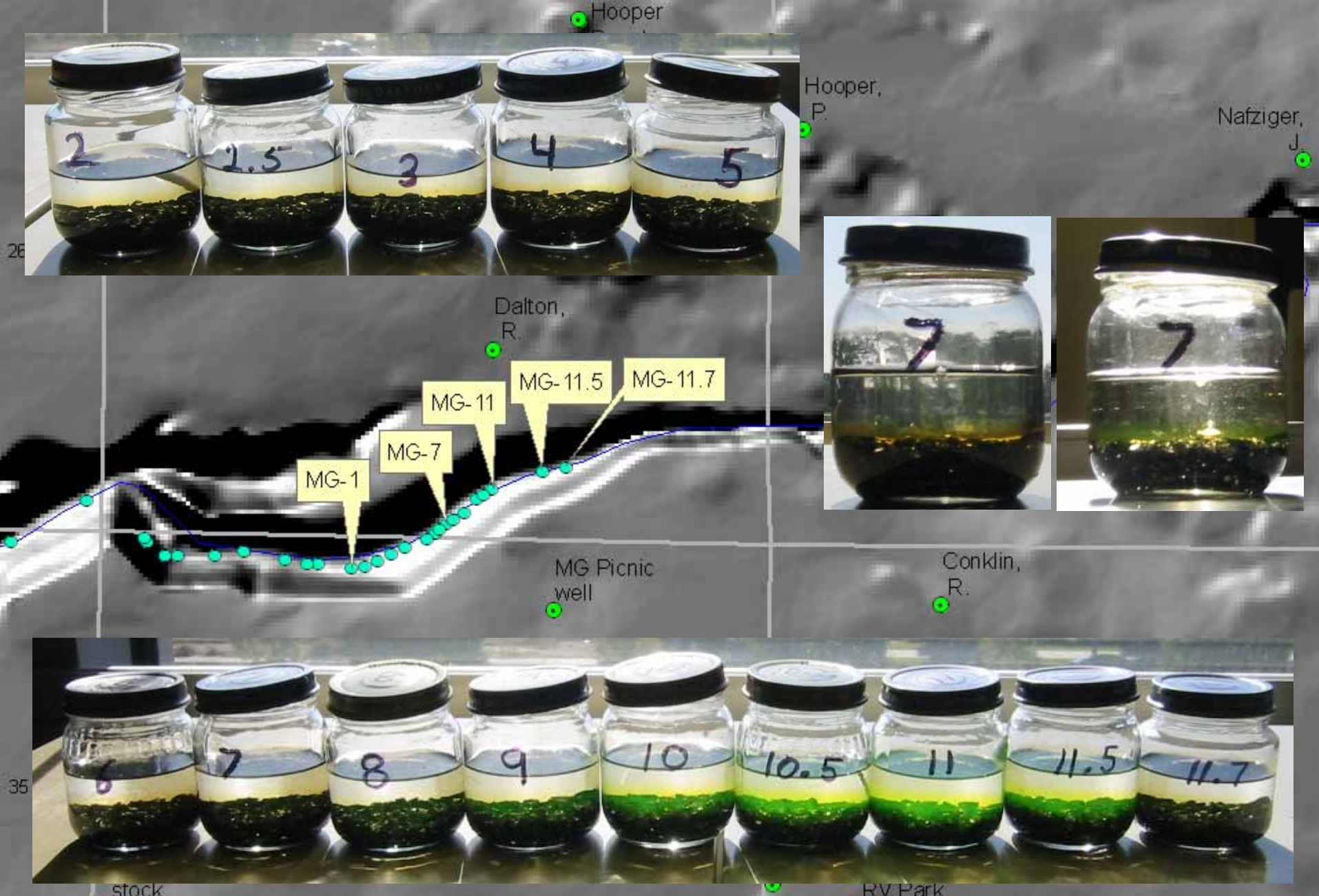
Figure 31. Charcoal packet results for Conklin well #52 Trace #2 visually showing green dye in MG-7 through 11.5. Placing the samples on a stainless steel surface improves visibility of the dye as seen in the right image of sample #7 comparison.
