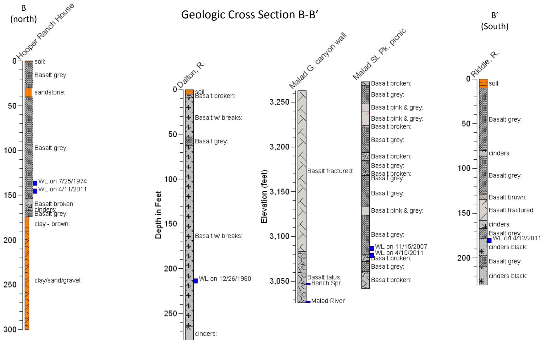
Figure 26. Geologic cross section B-B' showing basalt related rock types as grey background patterns and sediment related rock types as orange background patterns. Water levels symbols are blue. Note the lack of sediments near the Malad Gorge at these depths compared to cross section A-A' east of the Gorge.
