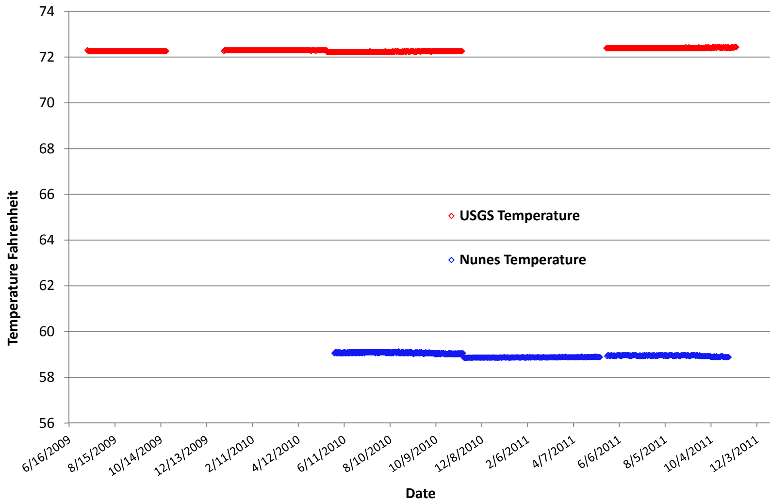
Figure 6. Temperature data for USGS Henslee well showing over 72 degree Fahrenheit water at 600 foot depth and the temperature for the 123 foot deep domestic well (Nunes D0023382) 60 feet south of the USGS well.
